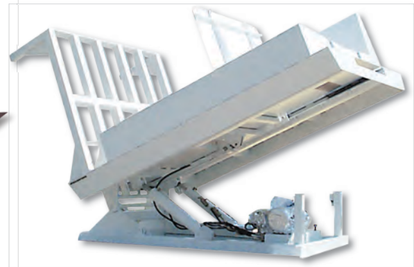
Customized Upender
